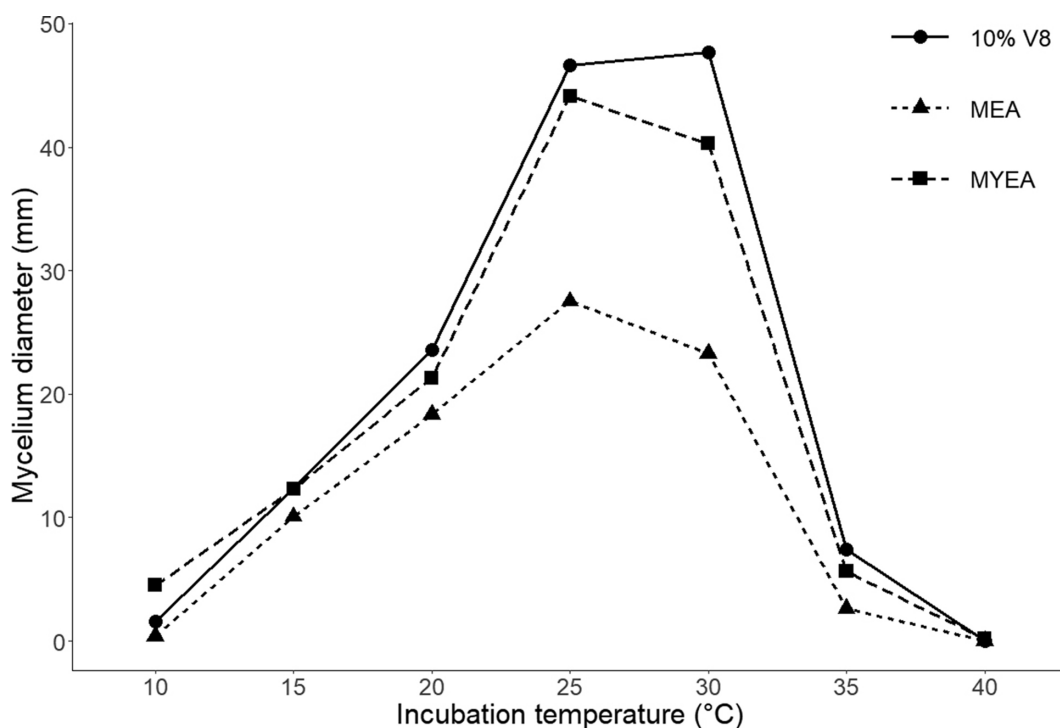
FIGURE 1. Diameter of colonies (in mm) of Ceratocystis lukuobia isolates grown on three different culture media at seven different temperatures. Measurements were taken 7 days post-inoculation.
