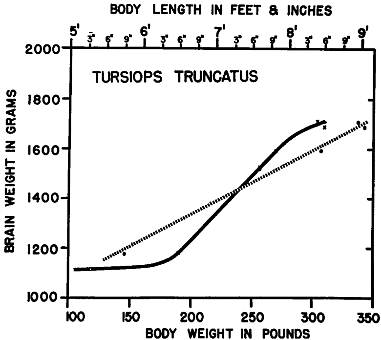
FIG. 1.—The bottlenose dolphin's brain weight is given on the left hand edge of the figure. The body weight versus the brain weight is the dotted curve. The solid curve is the body length versus the brain weight. It should be noted that the critical value of mammalian brain weight (900–1,000 gm.), which is the subject of this article, is below all values in this figure; all brains of bottlenose dolphins measured to date are above the critical threshold value.
