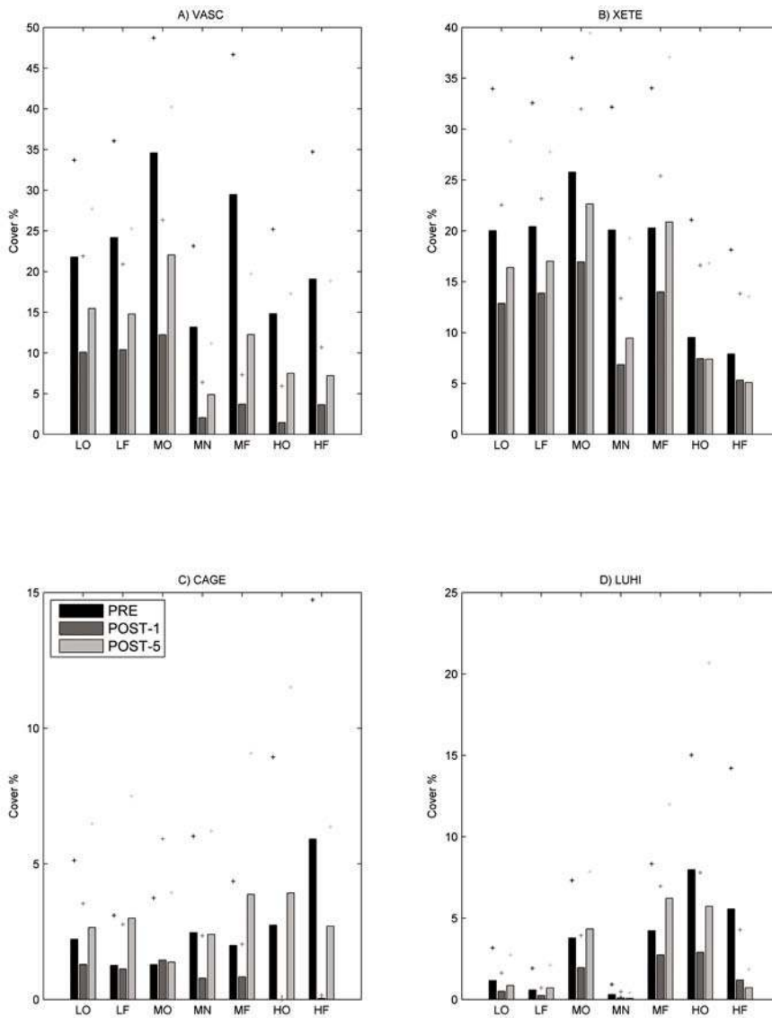
Figure 6. Canopy cover of the four dominant undergrowth plant species across each of the treatment combinations before treatment (PRE) and one year (POST-1) and five years (POST-5) after treatment: a) Vaccinium scoparium (VASC); b) Xerophyllum tenax (XETE); c) Carex geyeri (CAGE); and d) Luzula hitchcockii (LUHI). Treatment combination codes are described in Table 3. The symbol + represents standard error of the mean.
