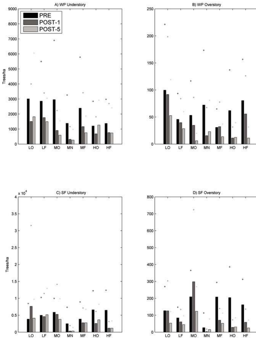
Figure 5. Tree density by species (WP, whitebark pine and SF, subalpine fir) and size class for each of the treatment combinations before treatment (PRE) and one year (POST-1) and five years (POST-5) after treatment. Treatment combination codes are described in Table 3. The symbol + represents standard error of the mean.
