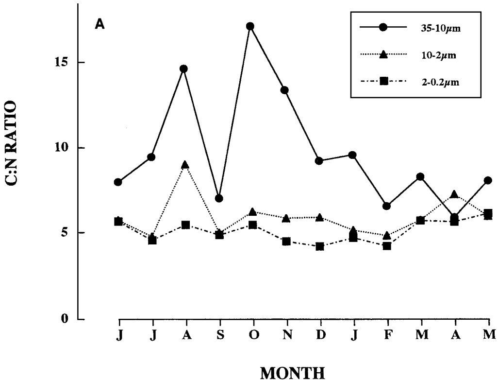
FIGURE 4. Seasonal variability in C:N ratios estimated from dark ^{14}\text{CO}_2 assimilation without enrichment for three size groups (A) and ammonium and phosphorus concentration (B) in Kāneʻohe Bay during the period from 16 June 1988 to 3 May 1989. When [C:N ratio] with enrichment was higher than [C:N ratio] in control, the nutrient limitation index was assumed as unity.
