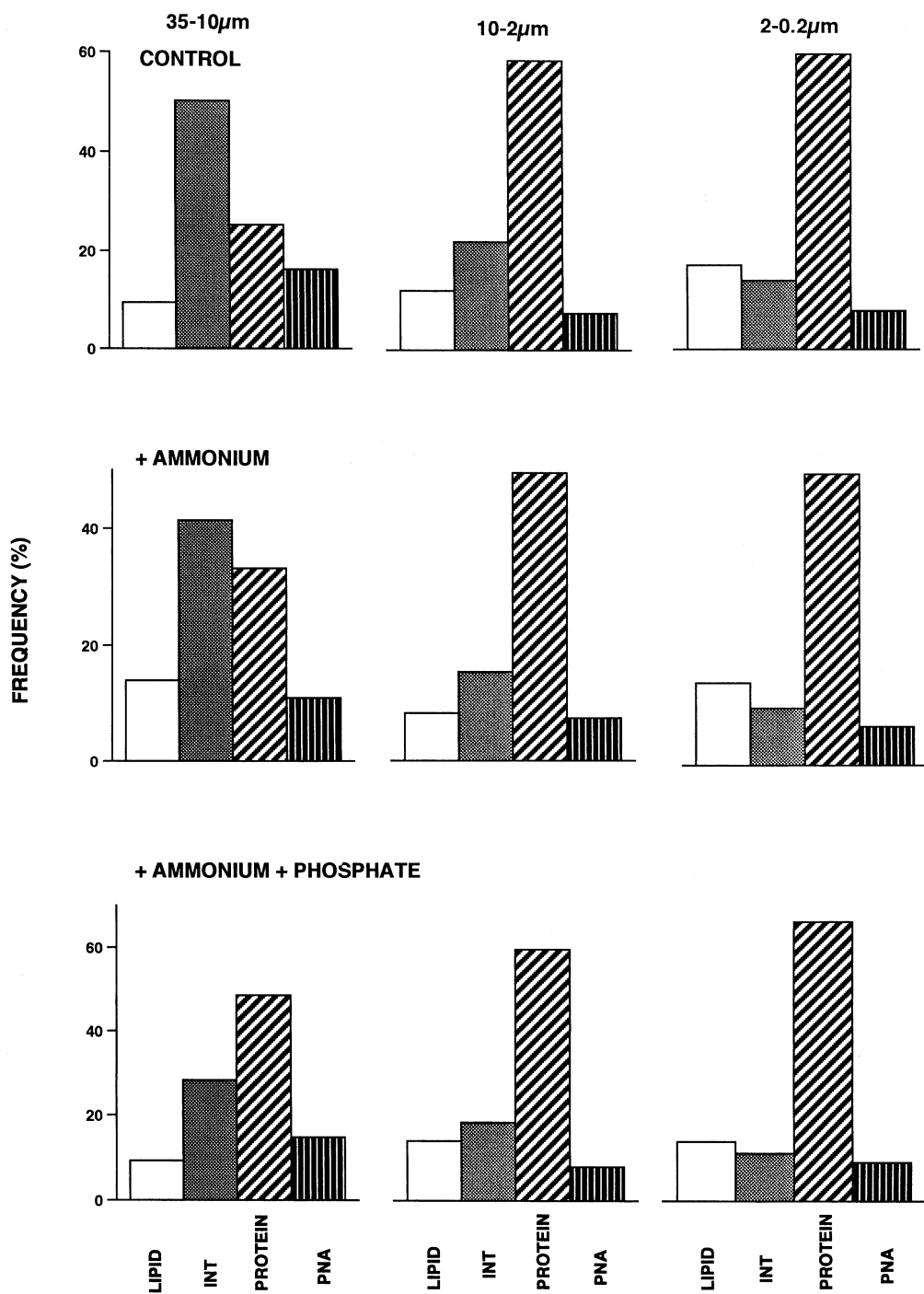
FIGURE 3. Relative distribution of ^{14}\text{CO}_2 incorporation into lipids, low-molecular-weight intermediate compounds (INT), protein, and polysaccharide plus nucleic acids (PNA) for the 35- to 10- \mu\text{m} , 10- to 2- \mu\text{m} , and 2- to 0.2- \mu\text{m} size groups of natural phytoplankton population without nutrients and with 3 \mu\text{M} of ammonium and 3 \mu\text{M} of ammonium plus 1 \mu\text{M} of phosphorus on 7 July 1988.
