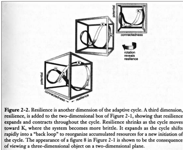
FIGURE 3. Resilience in the adaptive cycle. Source: Gunderson and Holling (2002, 41).
