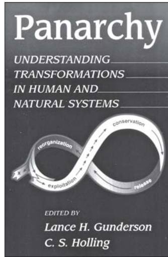
FIGURE 2. The adaptive cycle model. Source: Gunderson and Holling (2002, cover).
